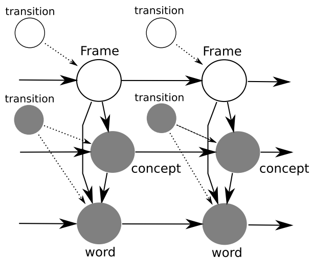
Figure 1: DBN-based semantic frame model. The model uses concept and word sequences as observation inputs for semantic frame decoding.
